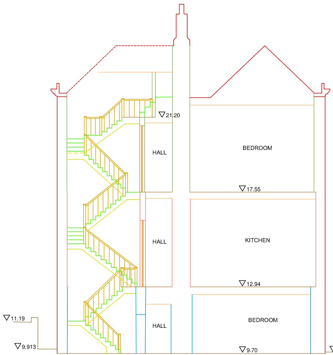
Cross Section Through Service Stairs Section 3
