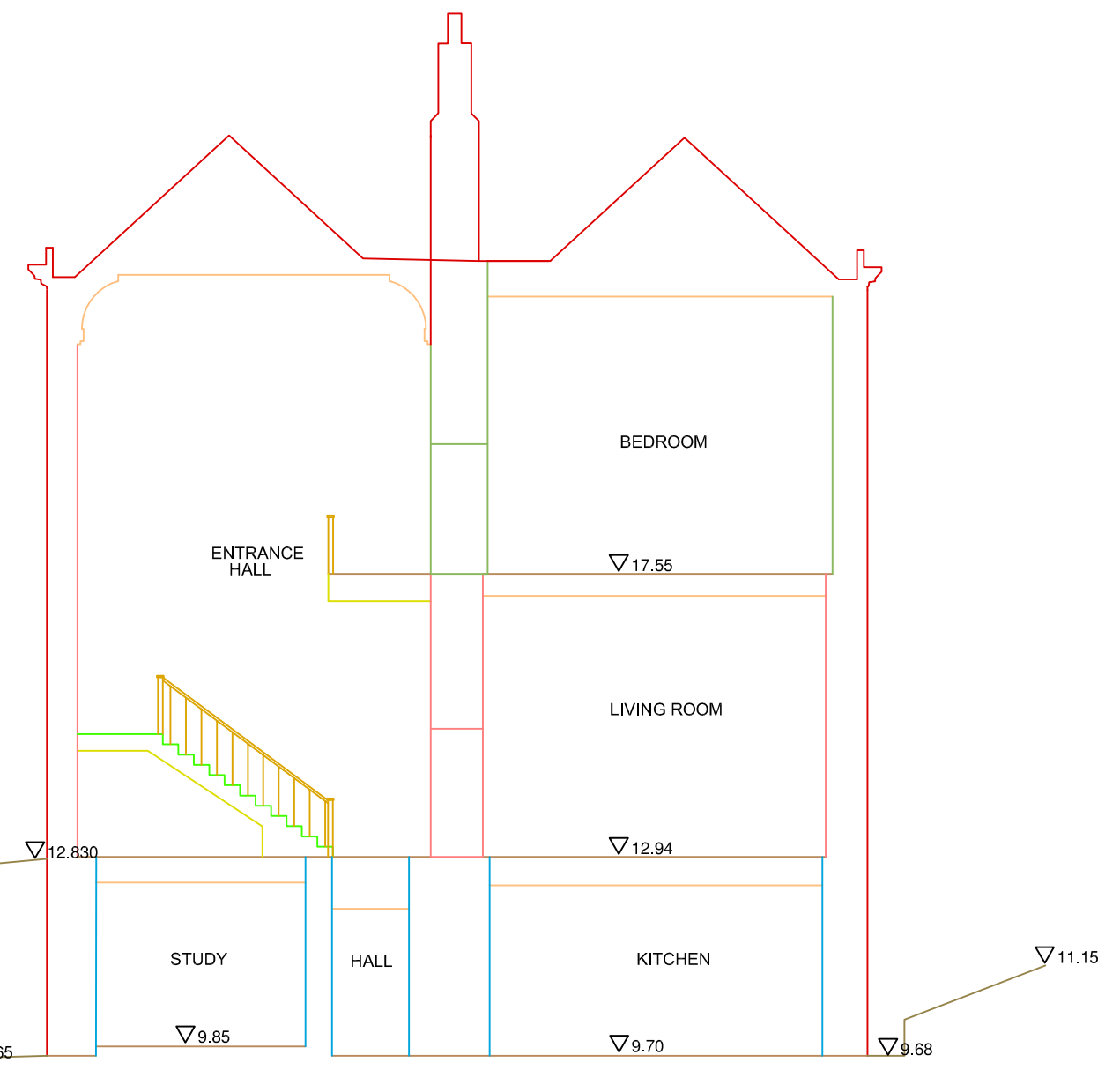
Cross Section Through Main Hall Stairs Section 4
